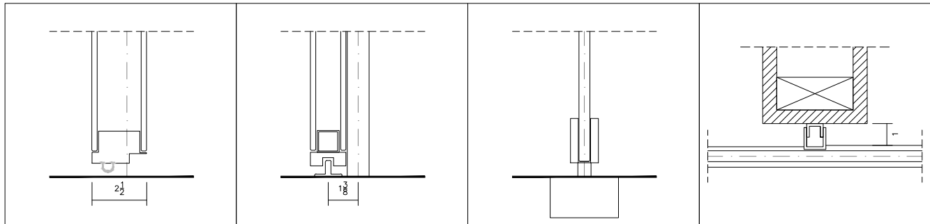
DOOR LEAF UNDERCUT W/ FLUSH DOUBLE-GLAZED DOOR
