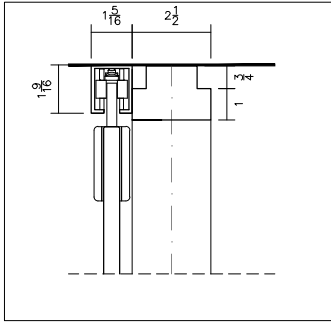
SLIDER TOP TRACK
