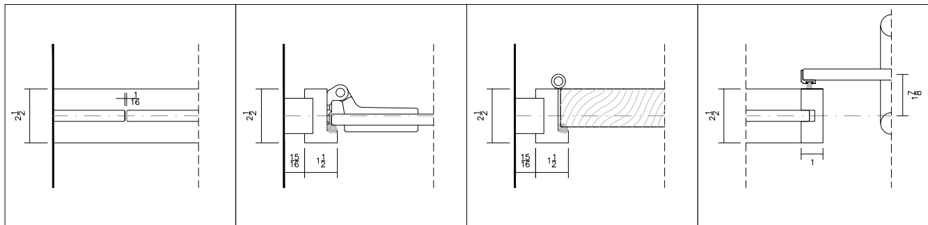
GLASS-TO-GLASS TYPICAL JOINT @ VHB CONNECTION
