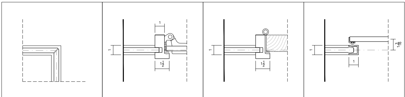
MITERED GLASS CORNER @ VHB CONNECTION
